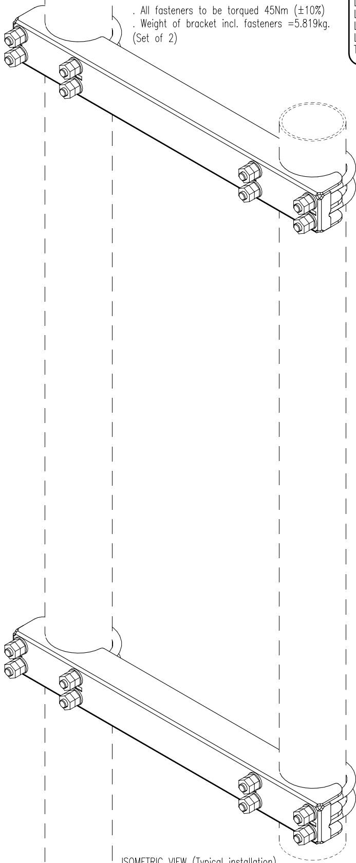
ISOMETRIC VIEW (Typical installation)
