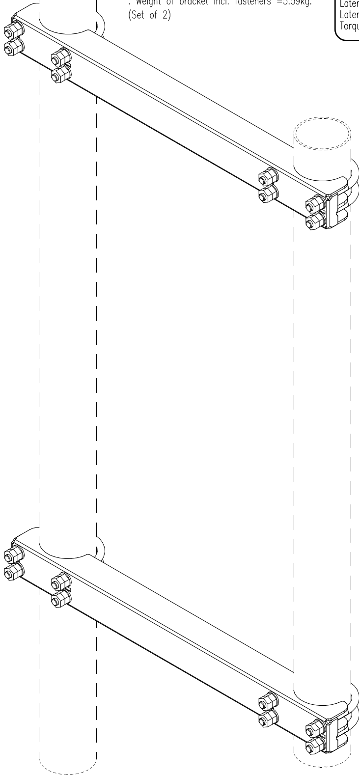
ISOMETRIC VIEW (Typical installation)
